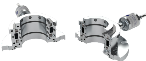
Split seal arangment for large shaft diameter
